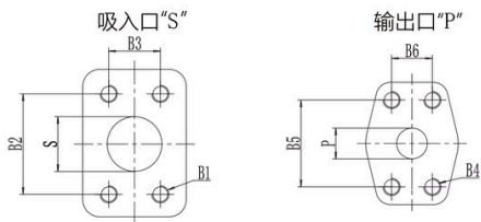
串泵油口法兰 Series Pump Oil Port Flange
